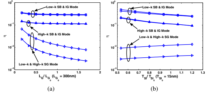
Fig. 6. (a) Variation of \eta vs. L_G/L_{G0} , L_{G0} = 300nm and (b) variation of \eta vs. T_{SI}/T_{SI0} , T_{SI0} = 15nm
