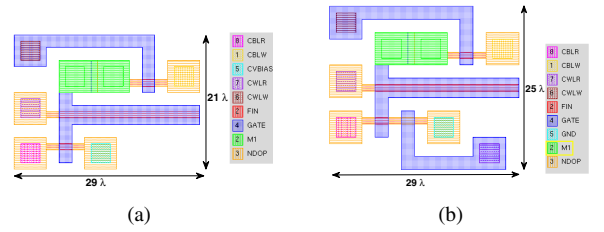
Fig. 16. (a) Layout of a Type 1 cell and (b) layout of a Type 3 cell
