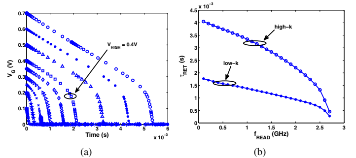
Fig. 13. (a) Retention period for a stored '1' for different V_{HIGH} at t = 0s in a low- k Type 1 cell with V_{WLR_{low}} = -0.3V and (b) \tau_{RET} vs. f_{READ} for low- k and high- k Type 1 cells
