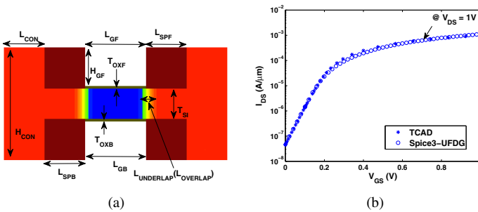
Fig. 4. (a) Two-dimensional (X-Y) cross-section of an n-FinFET simulated in Sentaurus TCAD and (b) I_{DS} vs. V_{GS} for V_{DS} = 1V simulated in Sentaurus TCAD and Spice3-UFDG
