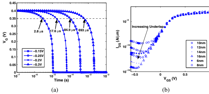
Fig. 15. (a) Retention time for a stored '1' at different V_{WLW_{low}} in a low- k Type 1 cell with V_{HIGH} = 0.4V and (b) I_{DS} vs. V_{GS} for TW showing the role of underlap in suppressing leakage
