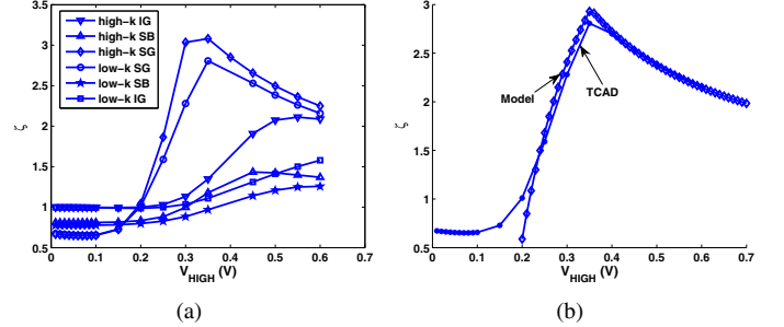
Fig. 8. (a) Variation of \zeta with TG in SG, SB and IG ( V_b = 0 ) modes vs. V_{HIGH} and (b) \zeta vs. V_{HIGH} for low- k SG-mode TG predicted by TCAD and the analytical model
