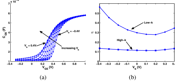
Fig. 7. (a) Shift in low- k IG mode C - V characteristics with V_b and (b) variation of \eta in IG mode vs. V_b
