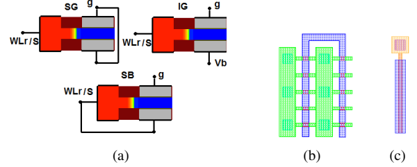
Fig. 5. (a) TG in SG, IG and SB modes, (b) layout of a multi-fin SG-mode TG , and (c) layout of a single-fin SG-mode TG
