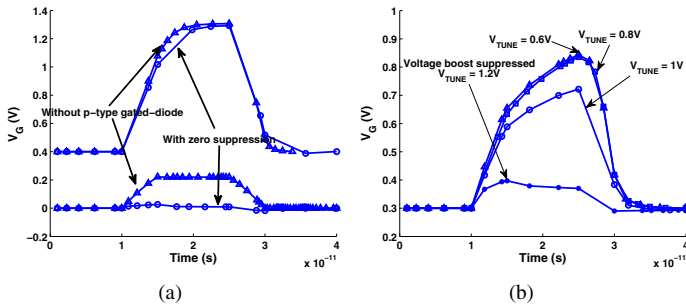
Fig. 22. (a) Voltage-boosting for V_{LOW} = 0V , V_{HIGH} = 0.4V , with and without zero-suppression and (b) tuning the voltage-boosting threshold with V_{TUNE} for V_{HIGH} = 0.3V
