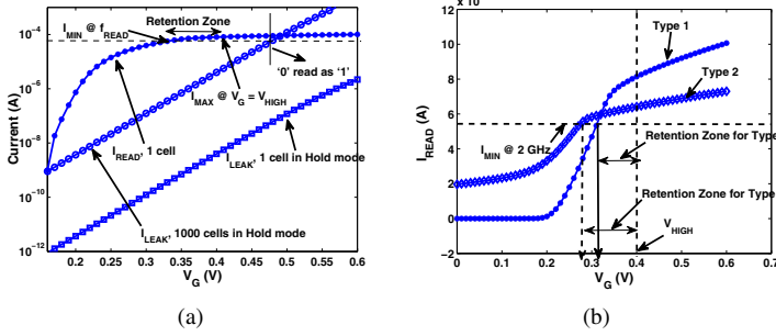
Fig. 14. (a) I_{READ} and I_{LEAK} vs. V_G , showing the retention zone for a low- k Type 1 cell and (b) I_{READ} vs. V_G , showing the retention zones for low- k Type 1 and 2 cells at f_{READ} = 2 GHz
