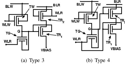
Fig. 11. Gated-diode 3T1D FinFET DRAM cells
