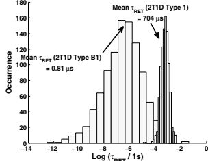
Fig. 17. Effect of process variations on \tau_{RET} of Type B1 cells at f_{READ} = 0.5 GHz and Type 1 cells at f_{READ} = 2.3 GHz
