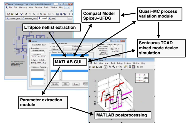
Fig. 3. FinE simulation framework for double-gate circuit design space exploration
