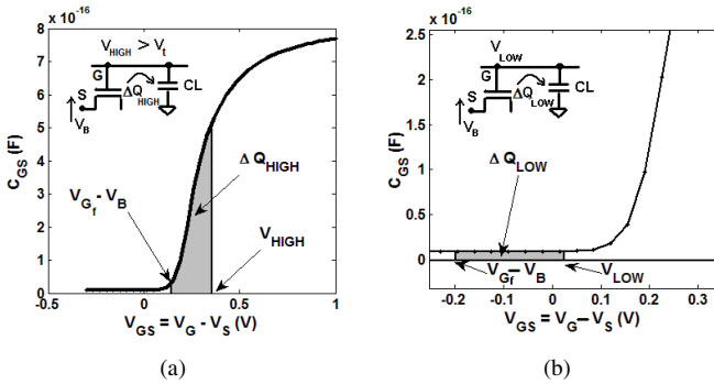
Fig. 2. \Delta Q_{HIGH} ( \Delta Q_{LOW} ) charge transferred when storage node G is at V_{HIGH} ( V_{LOW} ) and node S is raised by V_B
