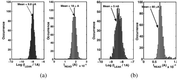
Fig. 18. (a) Effect of process variations on I_{LEAK} and I_{READ} for Type B1 cells and (b) effect of process variations on I_{LEAK} and I_{READ} for Type 1 cells
