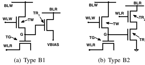
Fig. 1. Bulk gated-diode DRAM cells: (a) 2T1D and (b) 3T1D
