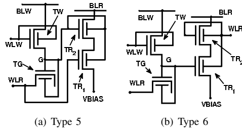
Fig. 12. Gated-diode 3T1D FinFET DRAM cells
