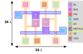
Fig. 19. Layout of an all-single-fin 6T FinFET SRAM with pass-gate feedback. Cell area \sim 0.26\mu m^2
