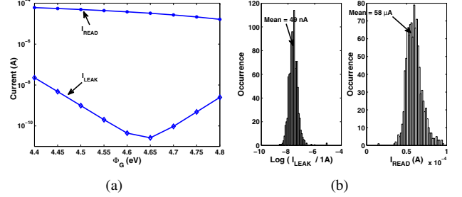
Fig. 20. (a) Variation of I_{READ} and I_{LEAK} with \Phi_G for 6T PGFB cells and (b) effect of process variations on I_{LEAK} and I_{READ} for 6T PGFB cells
