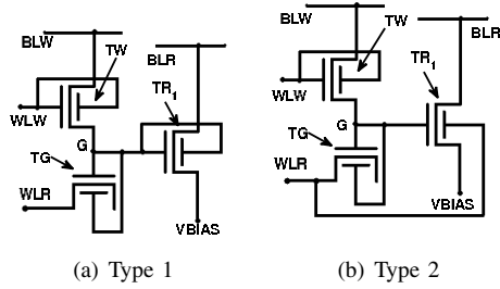
Fig. 10. Gated-diode 2T1D FinFET DRAM cells
