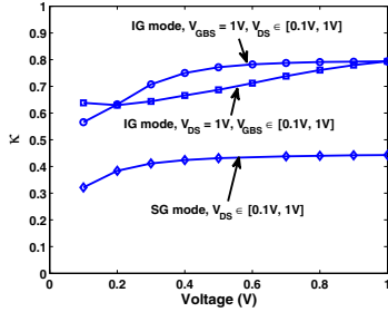
Fig. 9. Variation of \kappa_{low-k} in SG and IG modes under various biasing conditions, V_{HIGH} = 0.4V
